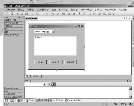
SharpDevelopのIDE
